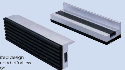
Aluminium base Rubber coating Jaws protection for vice
